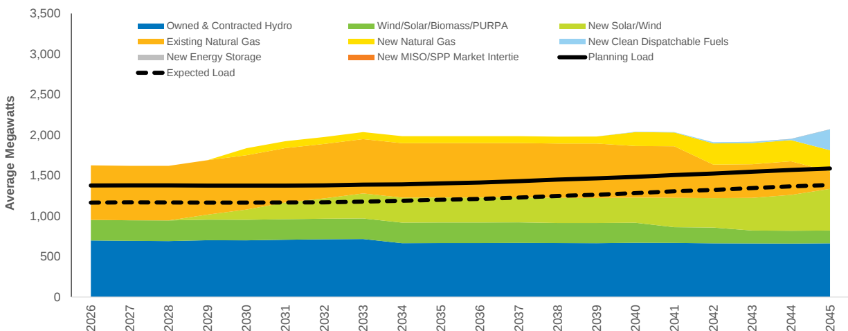
Figure 2.7: System Annual Energy Load & Resources
