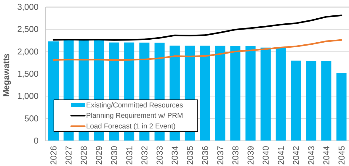
Figure 3: January Peak Load and Resource Position
